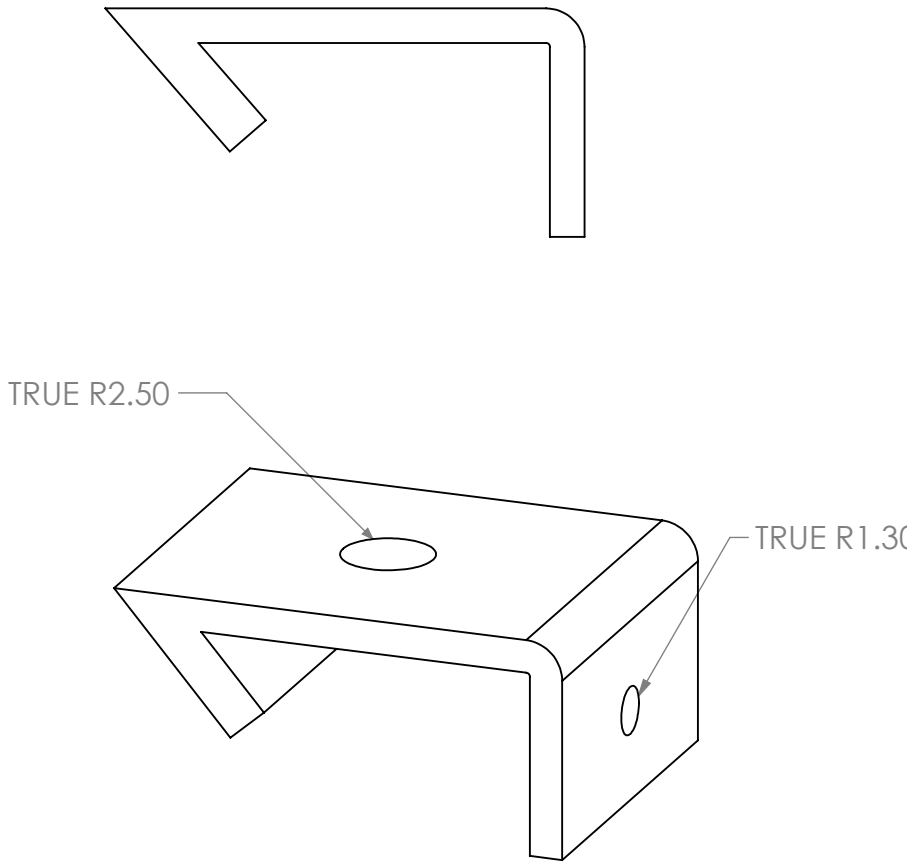
2. Ceiling Bracket
