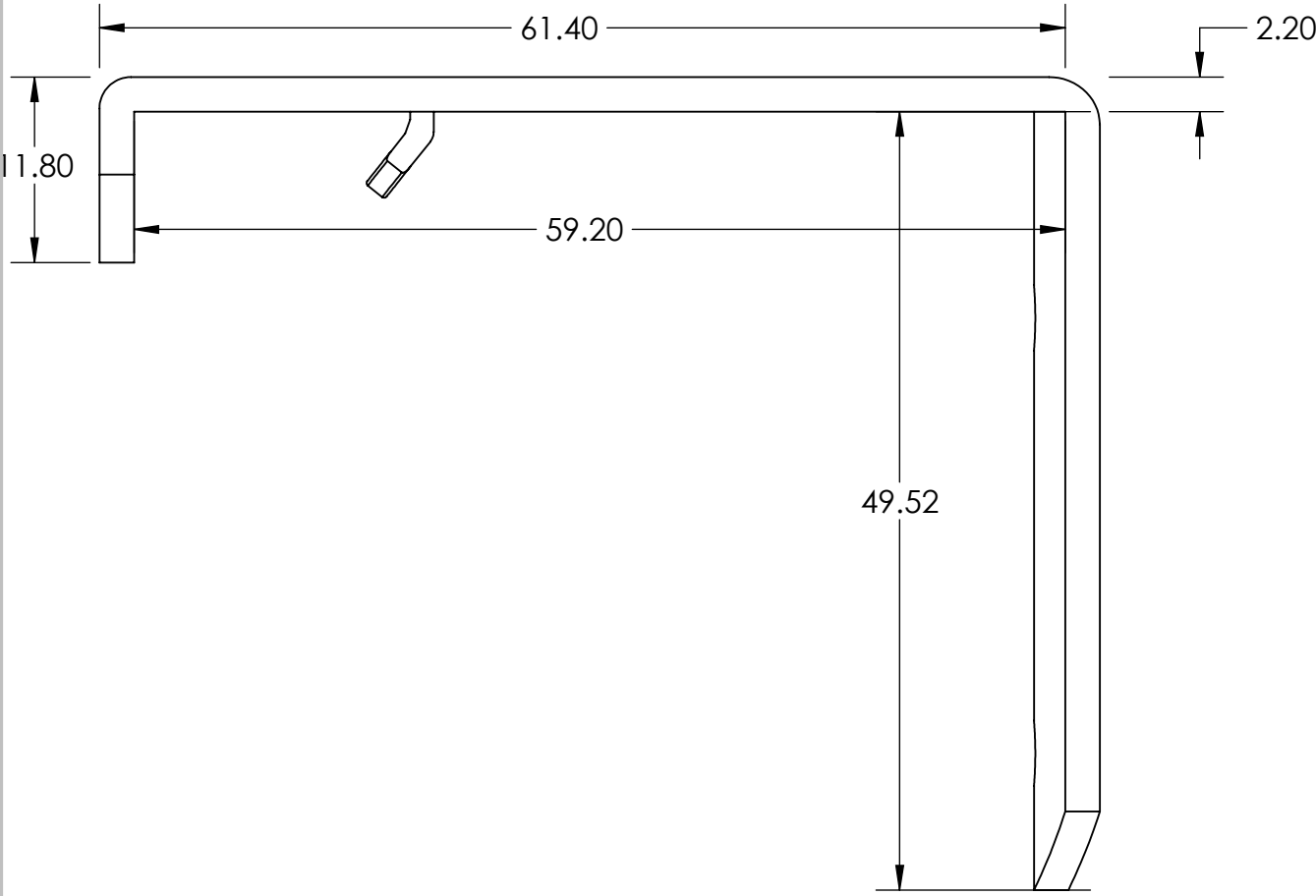
1. Wall Bracket
