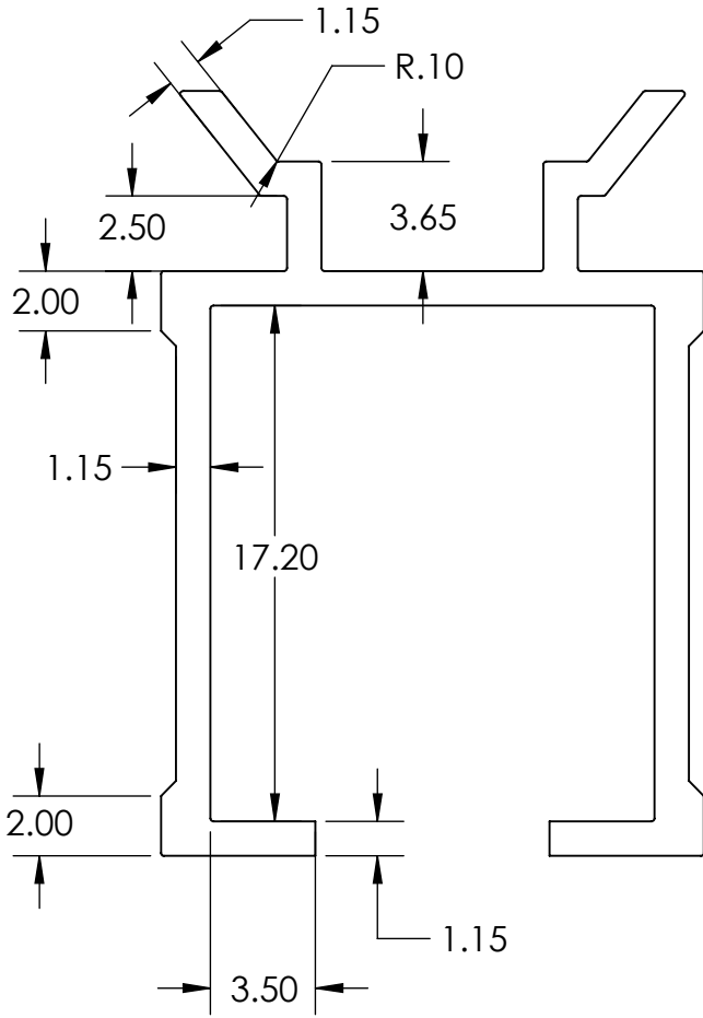
4. Runner
